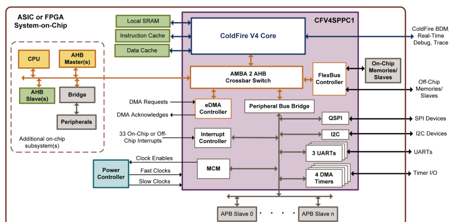
Example SoC Using CFV4SPPC1.
