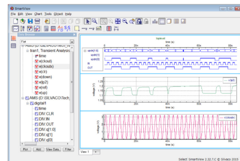
PLL- SPICE & Verilog-AMS mixed signal.
