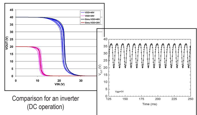
Comparison for an oscillator (Transient operation)
