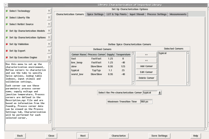
Viola characterization setup wizard.
