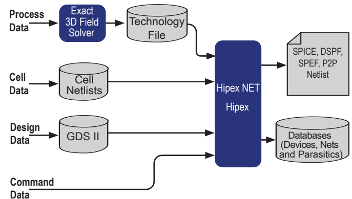
Hipex Full-Chip Parasitic Extractor Product Design Flow.
