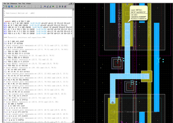
Hipex RC database provides visualization of parasitic elements on Expert layout view.
